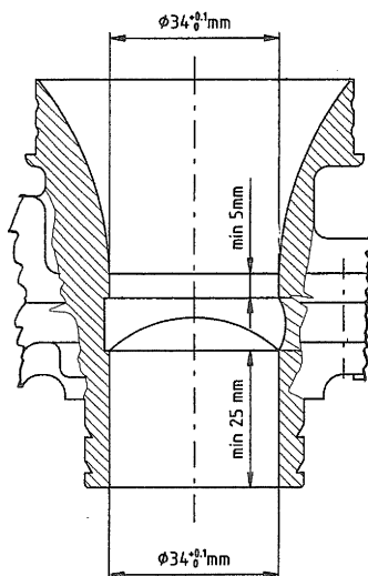
CARBURETTOR SECTION PLAN CARBURATEUR
