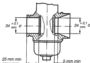
CARBURETTOR SECTION PLAN CARBURATEUR
