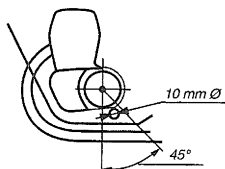
OPEN TRANSMISSION GUARDS
