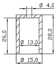
SPIKE GAUGE
